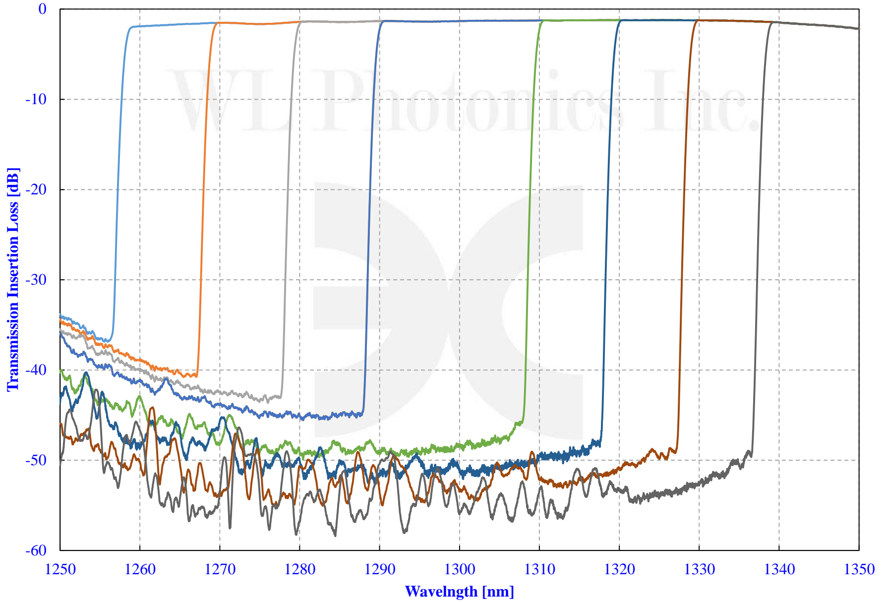
Transmission Spectrum of S-Grade Long Banspass Tunable Filter over 1260-1360nm
